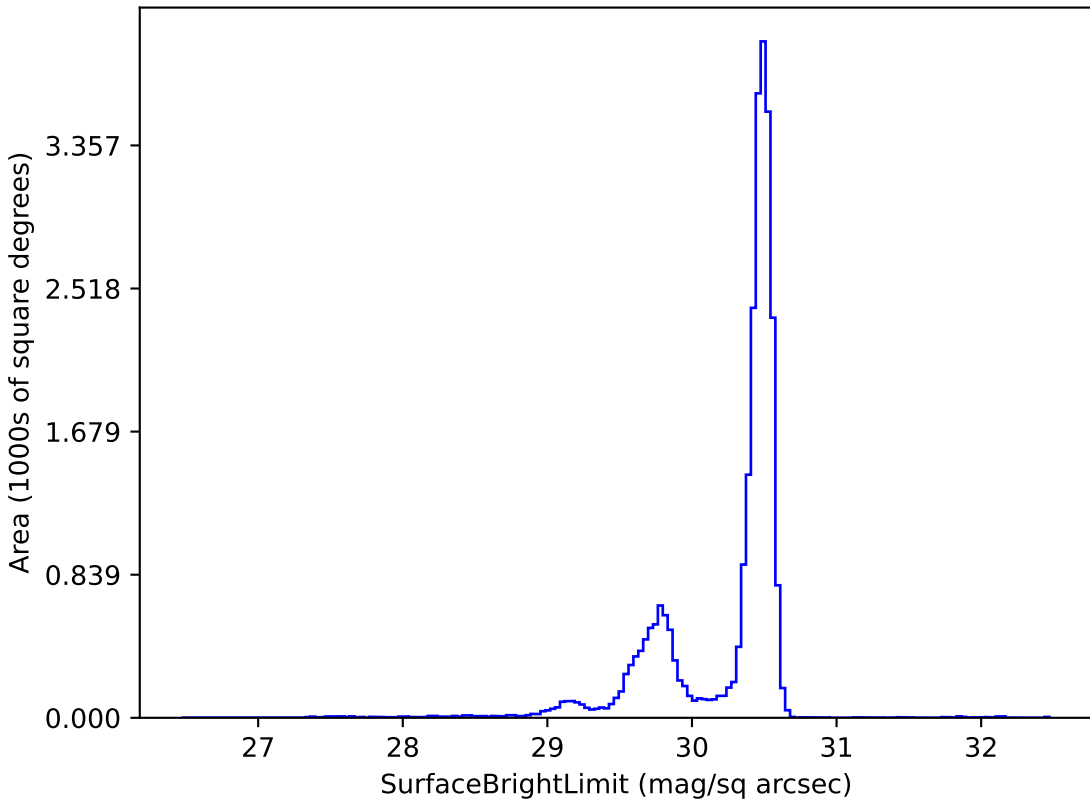
too_10_1v3.4_10yrs r: SurfaceBrightLimit
