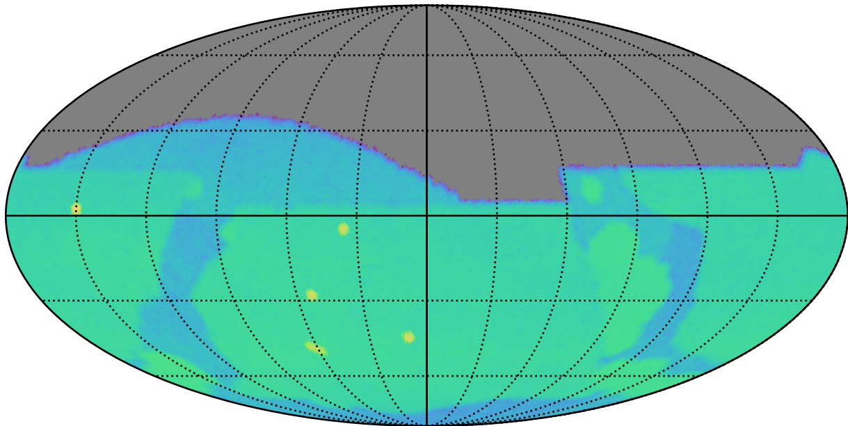
too_10_1v3.4_10yrs g: SurfaceBrightLimit
