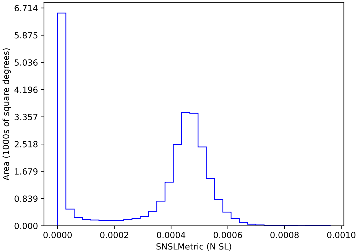
too_10_1v3.4_10yrs : SNSLMetric
