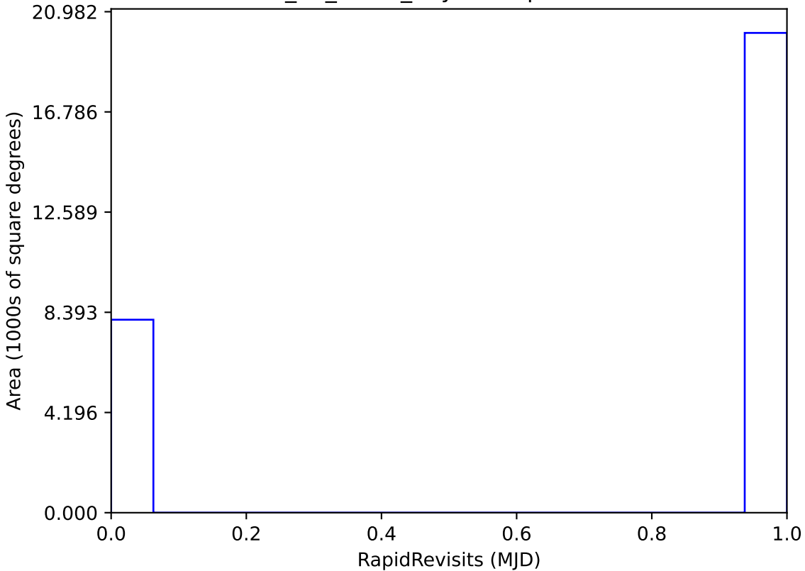
too_10_1v3.4_10yrs : RapidRevisits
