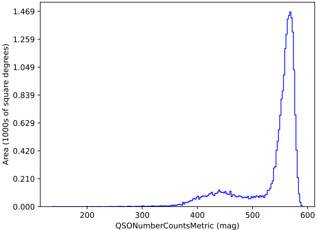
too_10_1v3.4_10yrs y band and non-DD: QSONumberCountsMetric
