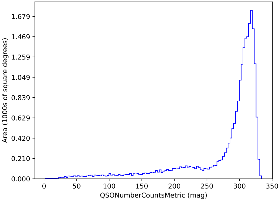
too_10_1v3.4_10yrs u band and non-DD: QSONumberCountsMetric
