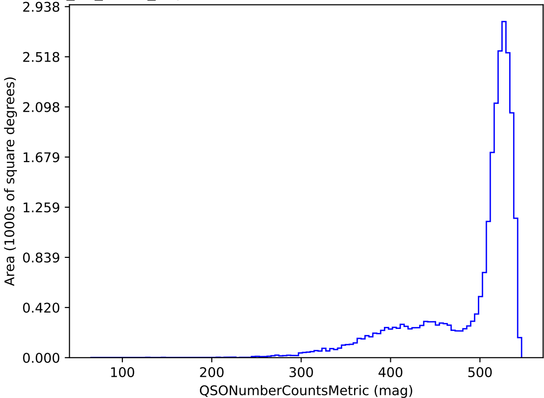
too_10_1v3.4_10yrs r band and non-DD: QSONumberCountsMetric
