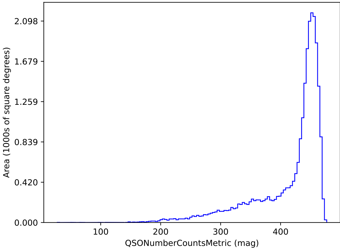
too_10_1v3.4_10yrs g band and non-DD: QSONumberCountsMetric
