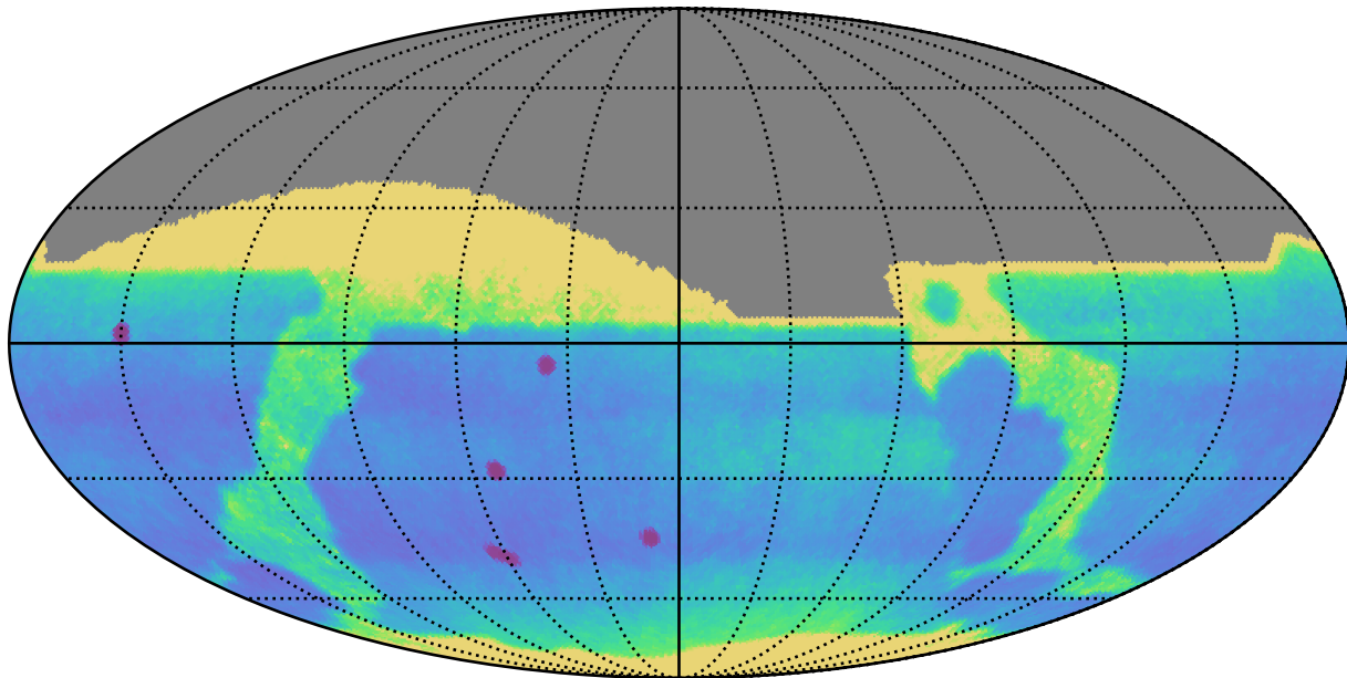
too_10_1v3.4_10yrs : Proper Motion Uncert @ 24.0
