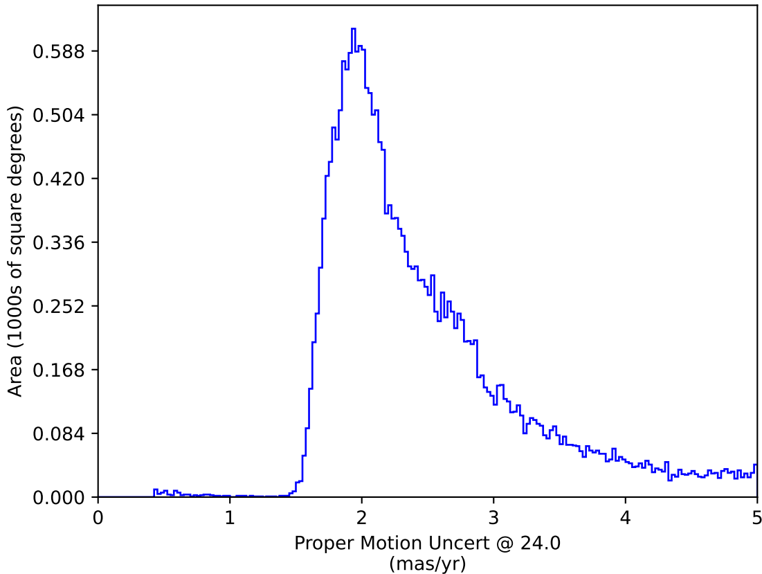
too_10_1v3.4_10yrs : Proper Motion Uncert @ 24.0
