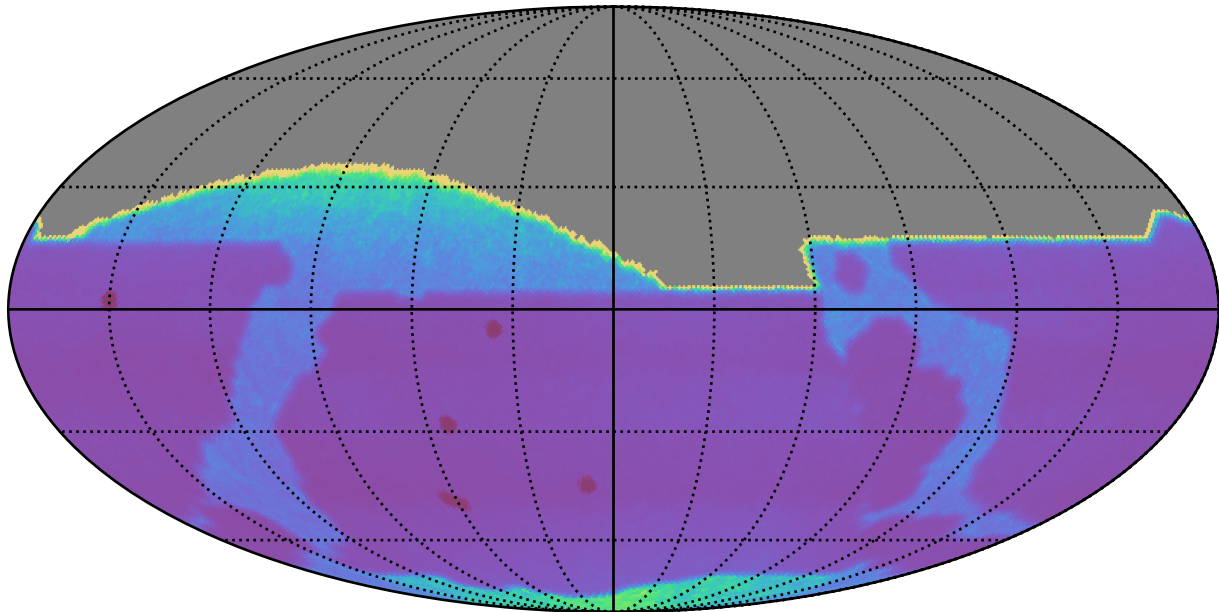
too_10_1v3.4_10yrs : Proper Motion Uncert @ 20.5
