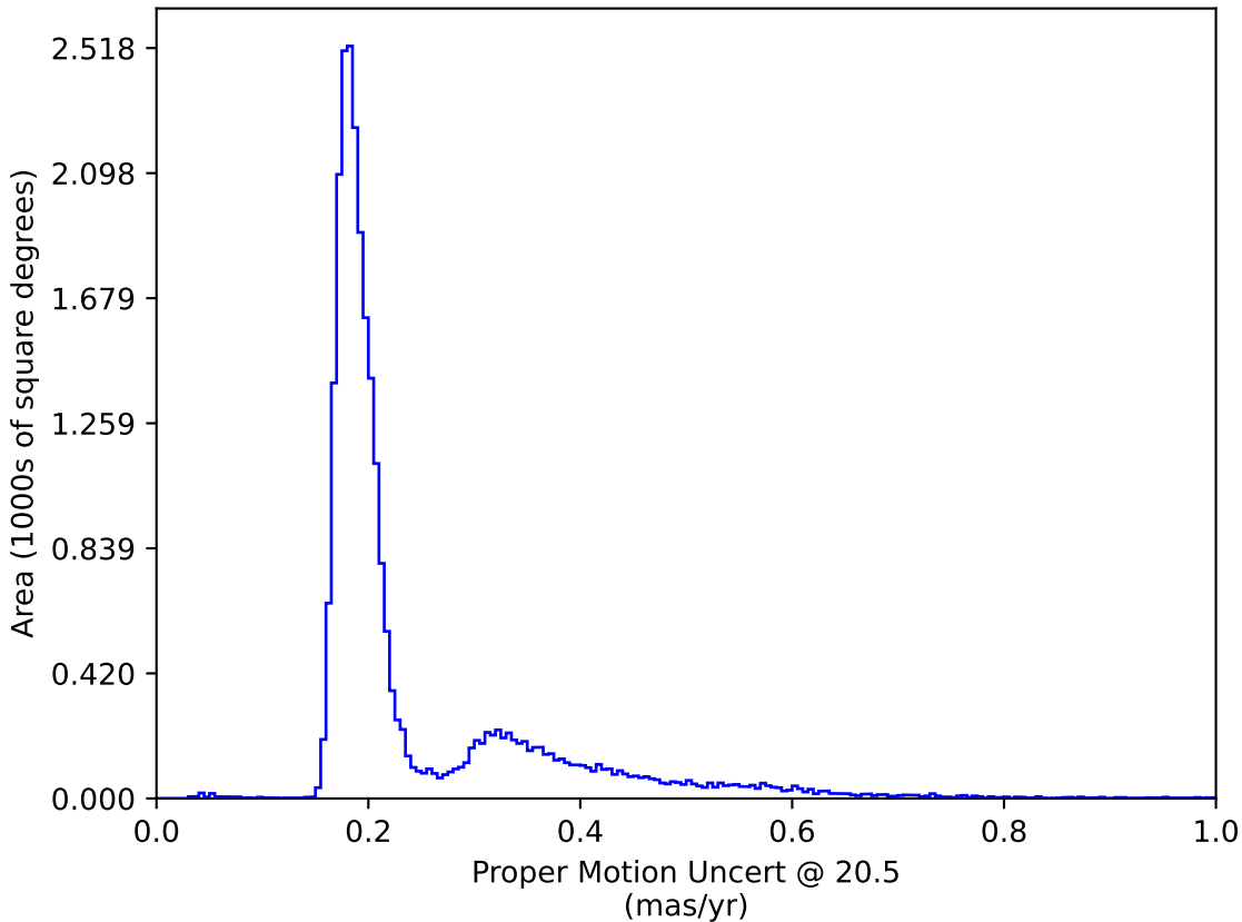
too_10_1v3.4_10yrs : Proper Motion Uncert @ 20.5
