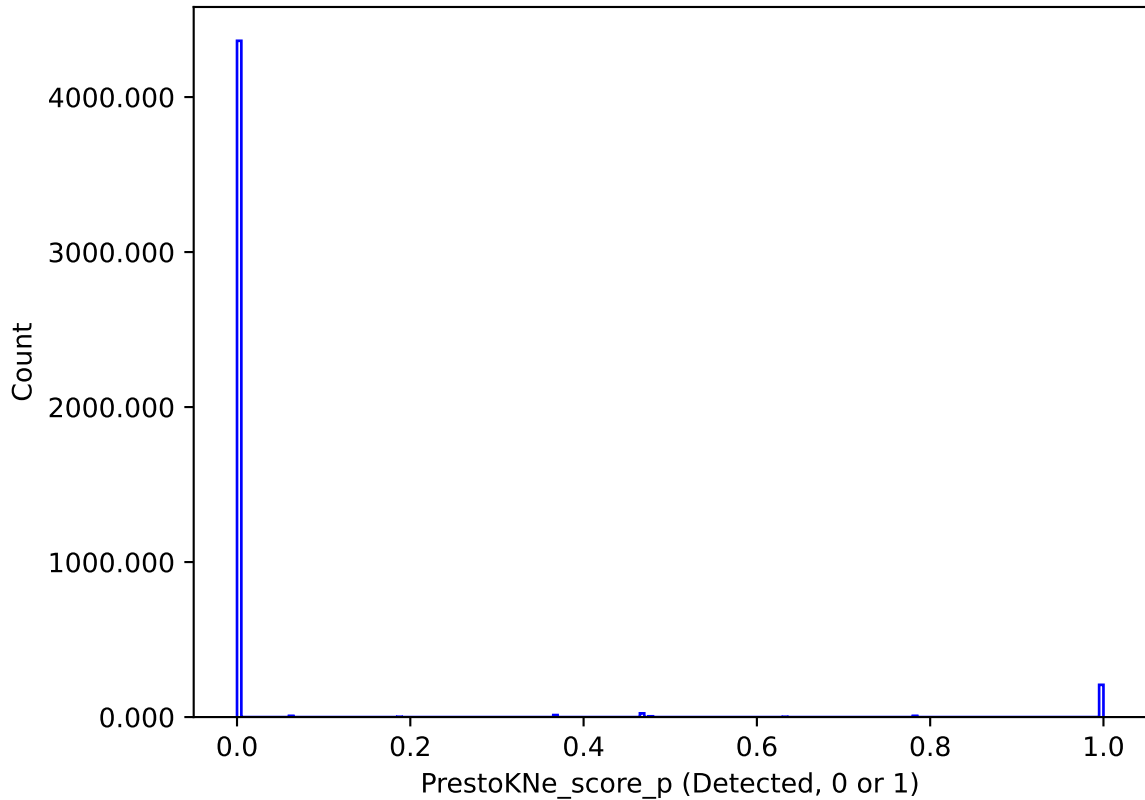
too_10_1v3.4_10yrs : PrestoKNe_score_p
