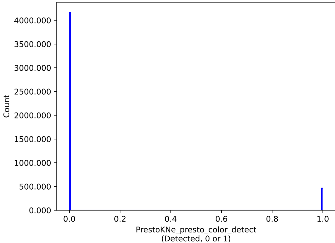
too_10_1v3.4_10yrs : PrestoKNe_presto_color_detect
