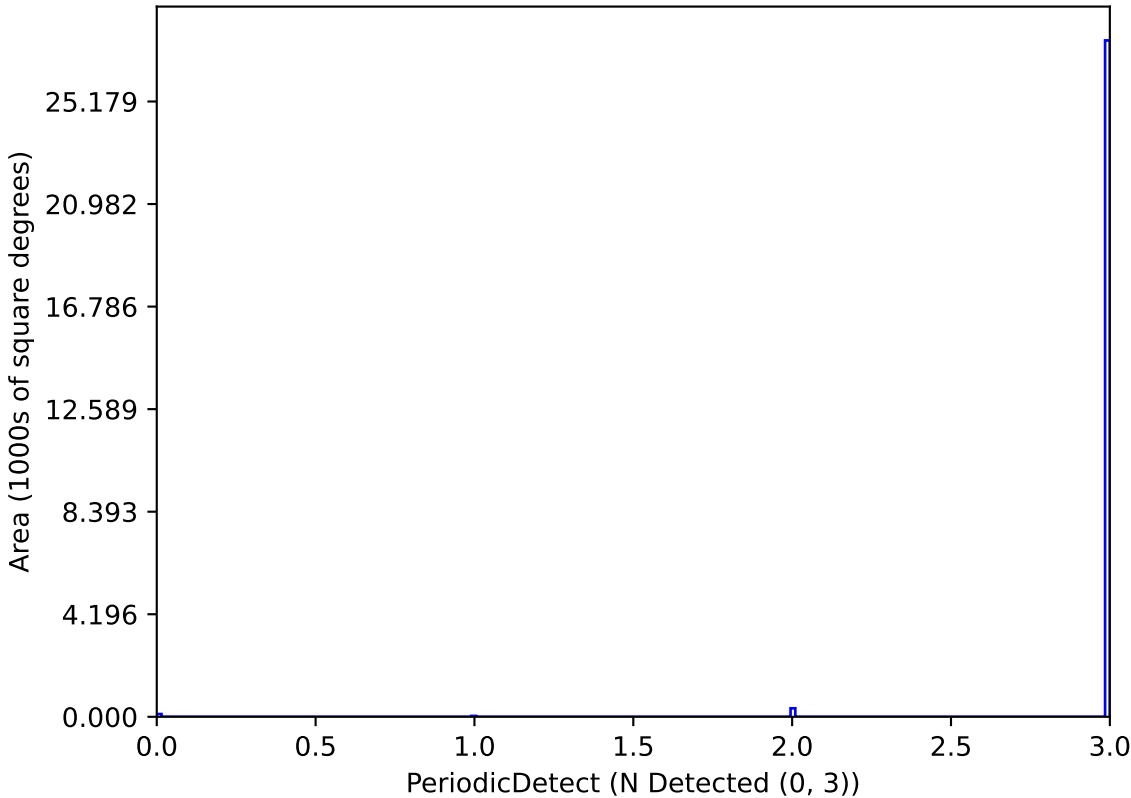
too_10_1v3.4_10yrs P_2.0_Mag_21_Amp_0.05-0.1-1: PeriodicDetect
