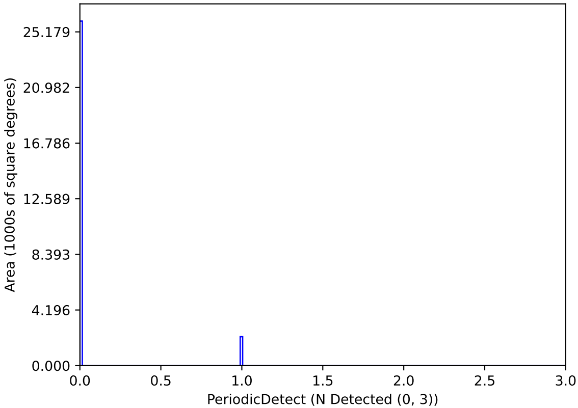
too_10_1v3.4_10yrs P_1.0_Mag_24_Amp_0.05-0.1-1: PeriodicDetect
