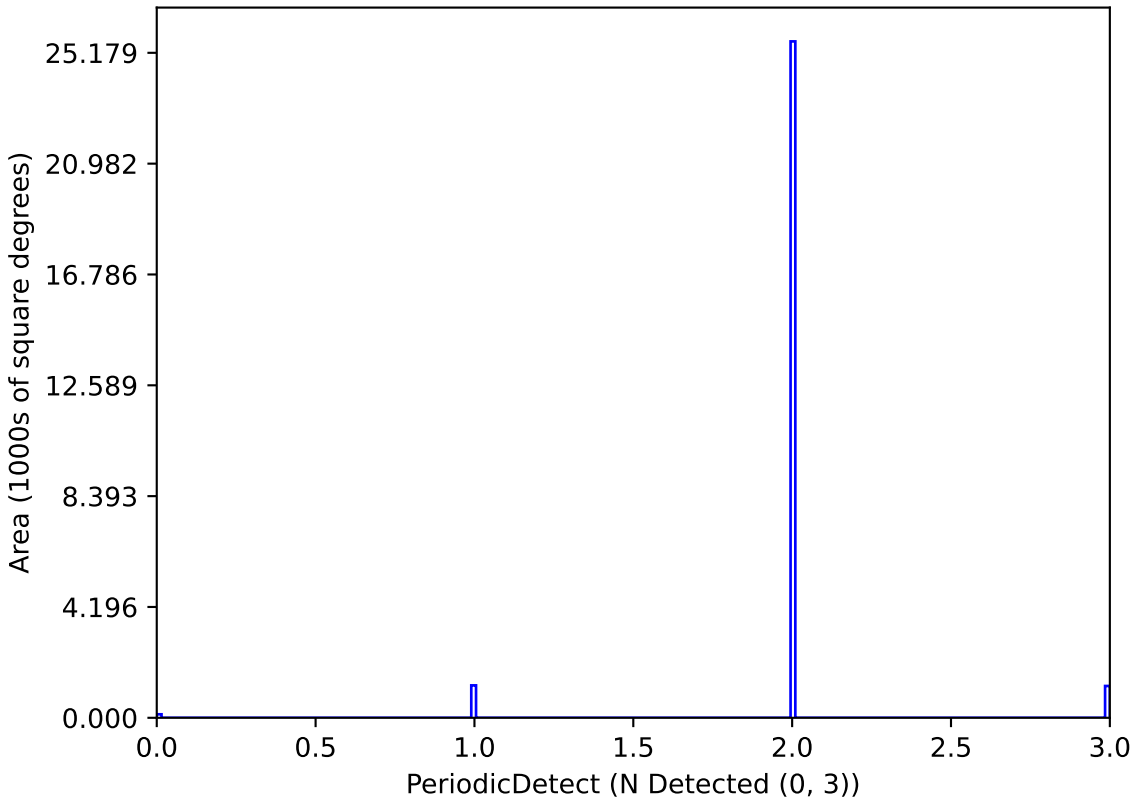
too_10_1v3.4_10yrs P_1.0_Mag_21_Amp_0.05-0.1-1: PeriodicDetect
