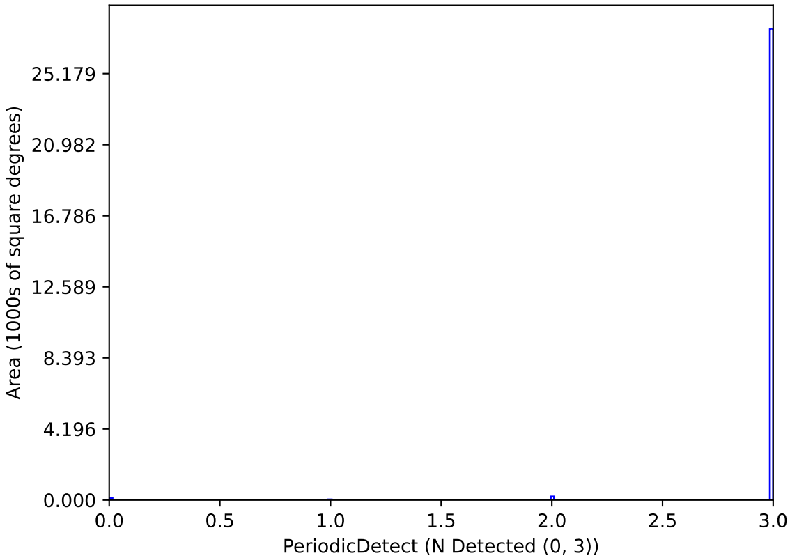
too_10_1v3.4_10yrs P_0.5_Mag_21_Amp_0.05-0.1-1: PeriodicDetect
