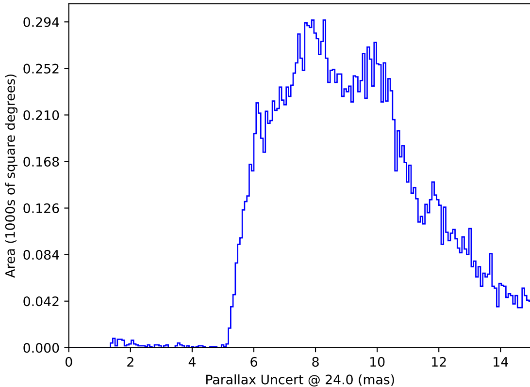
too_10_1v3.4_10yrs : Parallax Uncert @ 24.0
