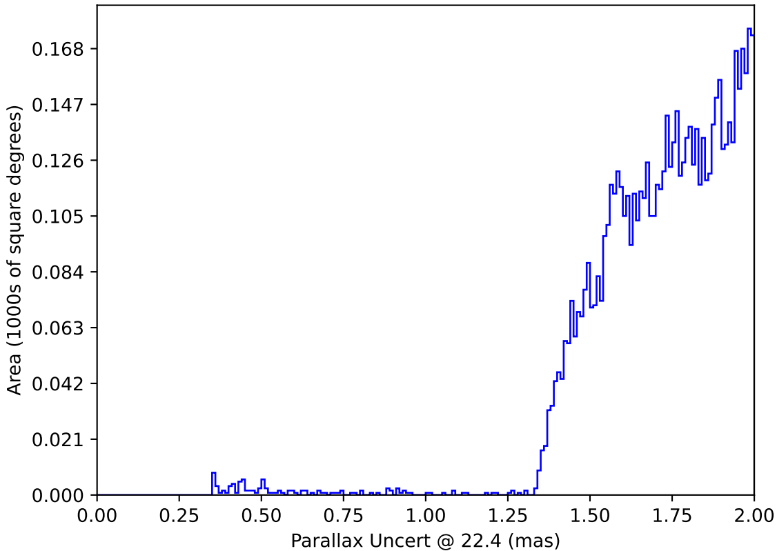
too_10_1v3.4_10yrs : Parallax Uncert @ 22.4
