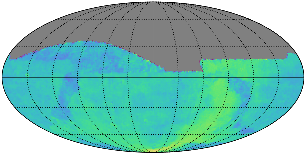
too_10_1v3.4_10yrs : Parallax Coverage @ 24.0
