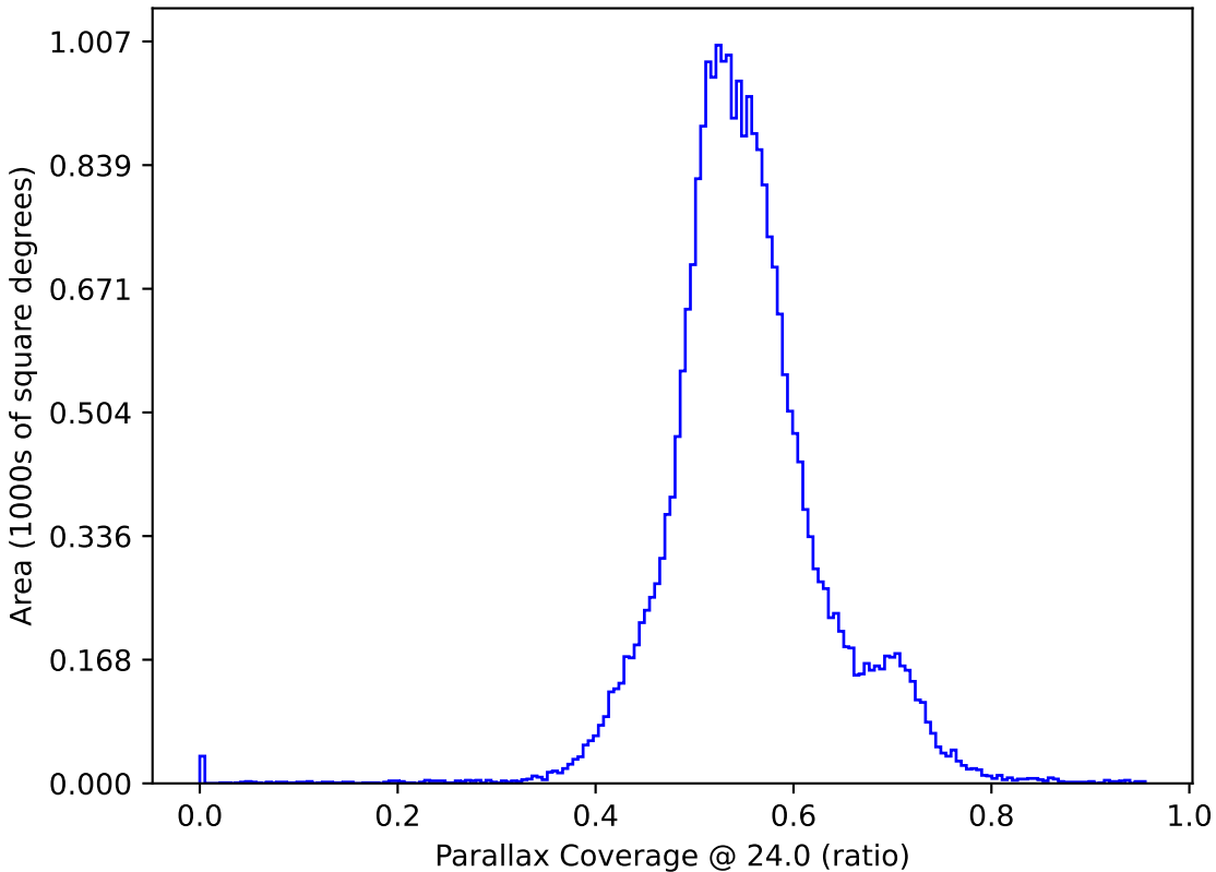
too_10_1v3.4_10yrs : Parallax Coverage @ 24.0
