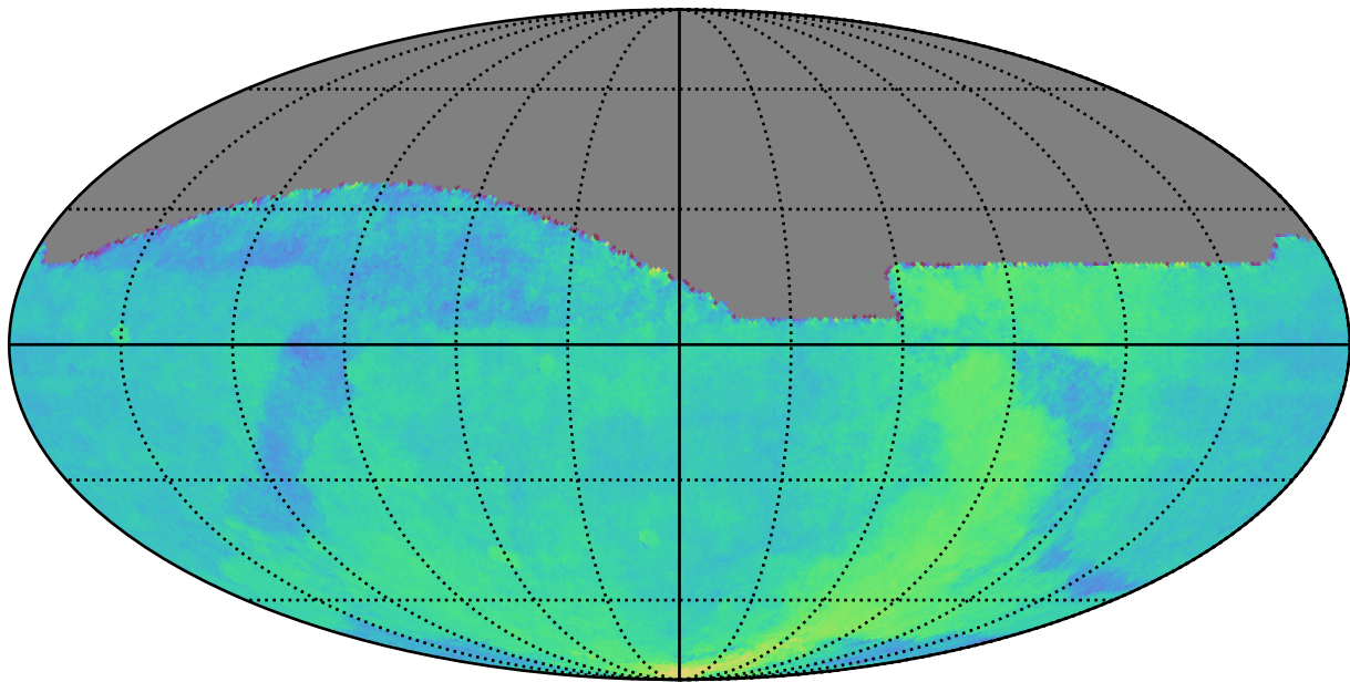
too_10_1v3.4_10yrs : Parallax Coverage @ 22.4
