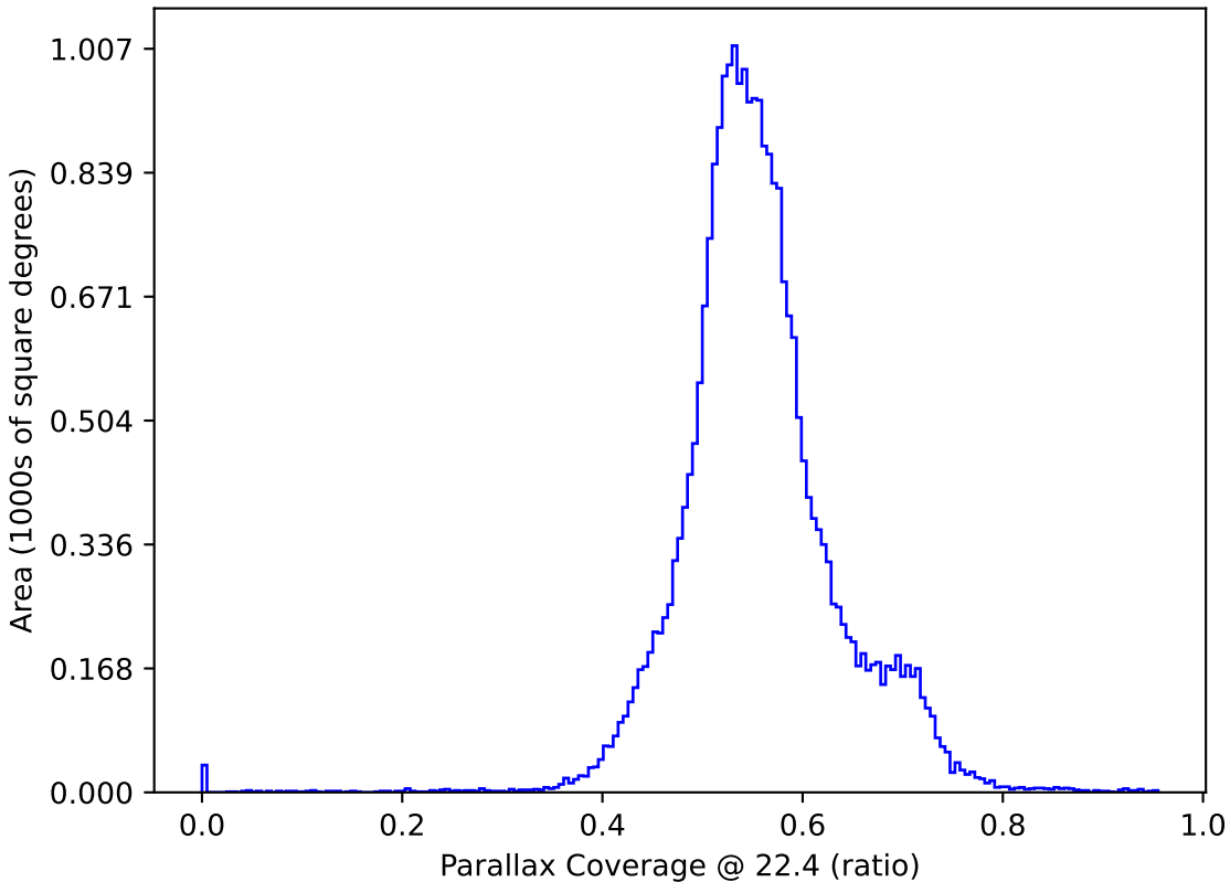
too_10_1v3.4_10yrs : Parallax Coverage @ 22.4
