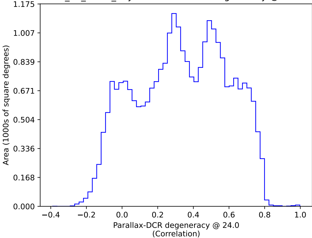
too_10_1v3.4_10yrs : Parallax-DCR degeneracy @ 24.0
