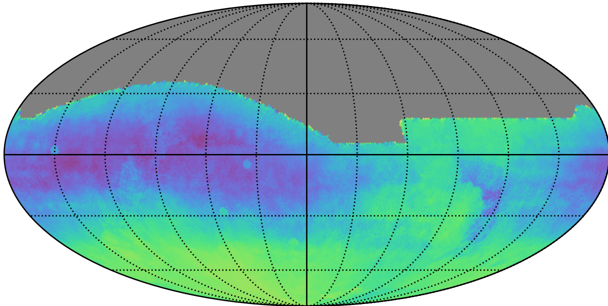
too_10_1v3.4_10yrs : Parallax-DCR degeneracy @ 22.4
