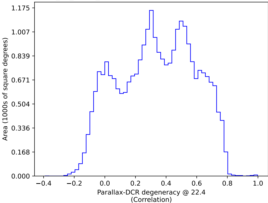
too_10_1v3.4_10yrs : Parallax-DCR degeneracy @ 22.4
