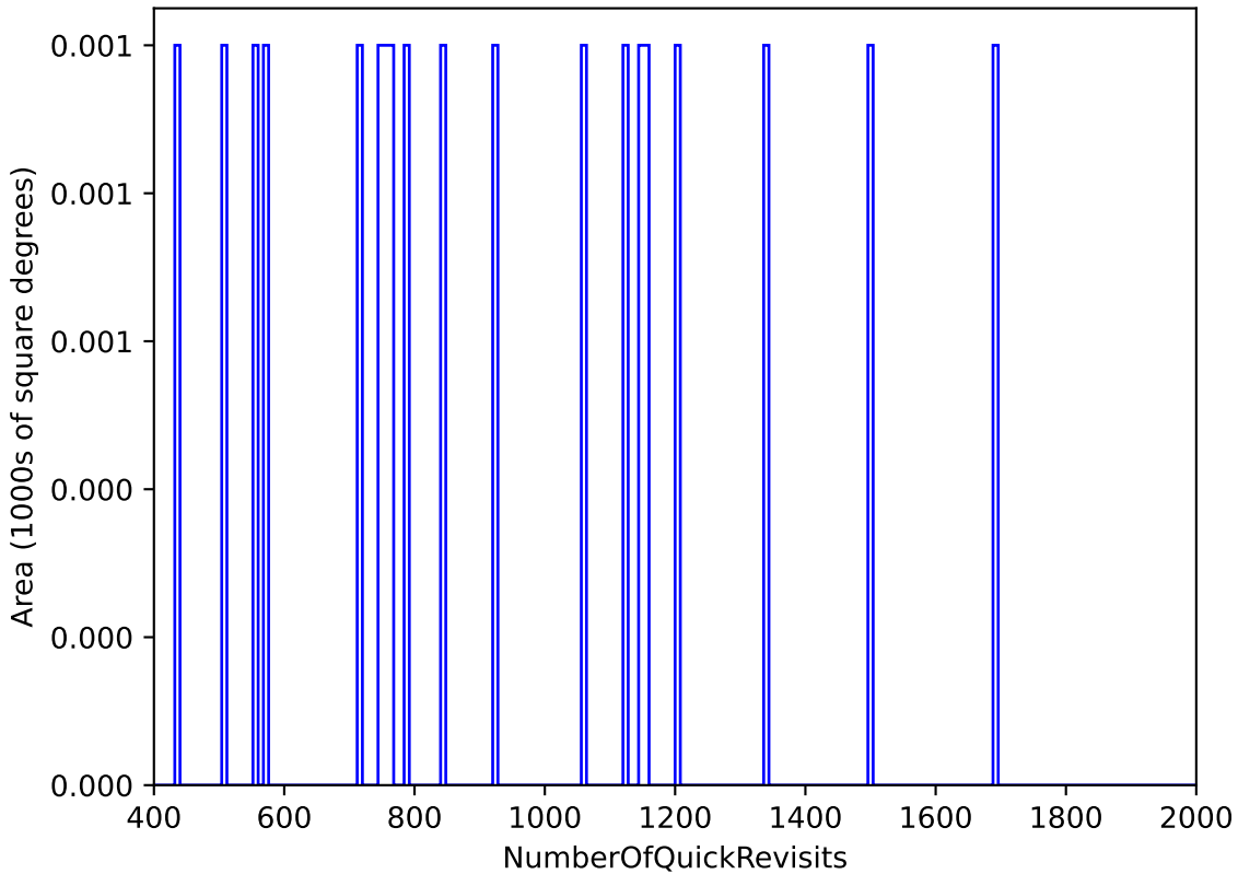
too_10_1v3.4_10yrs : NumberOfQuickRevisits
