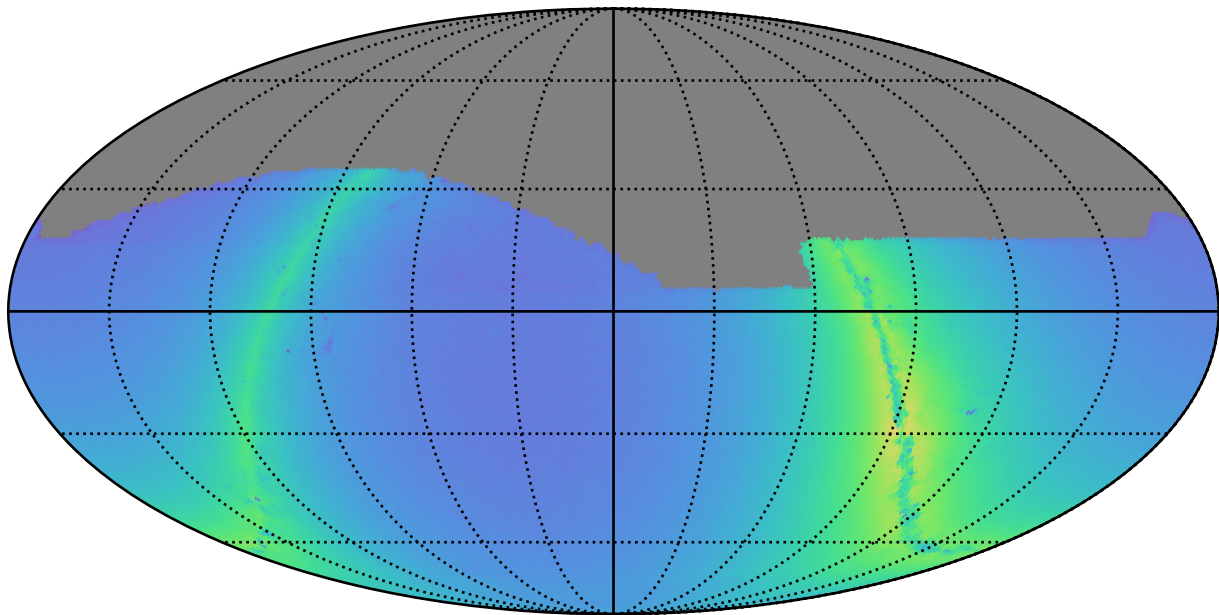
too_10_1v3.4_10yrs z: Nstars_no_crowding
