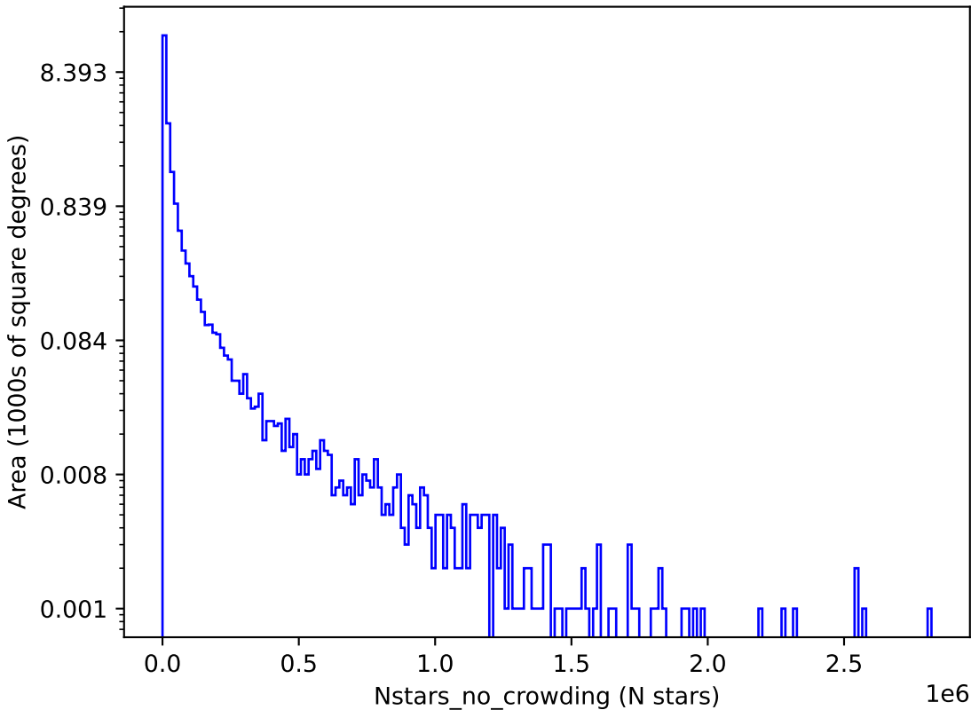
too_10_1v3.4_10yrs u: Nstars_no_crowding
