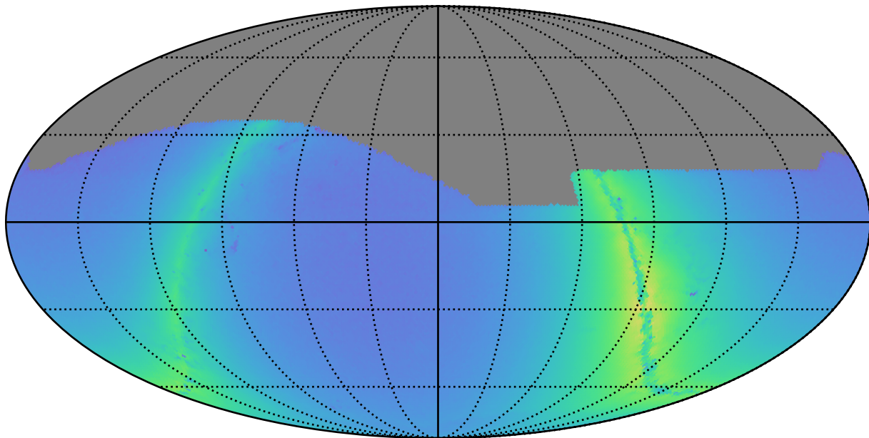
too_10_1v3.4_10yrs r: Nstars_no_crowding
