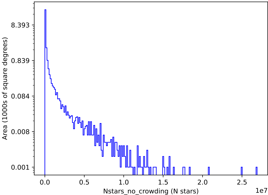
too_10_1v3.4_10yrs i: Nstars_no_crowding
