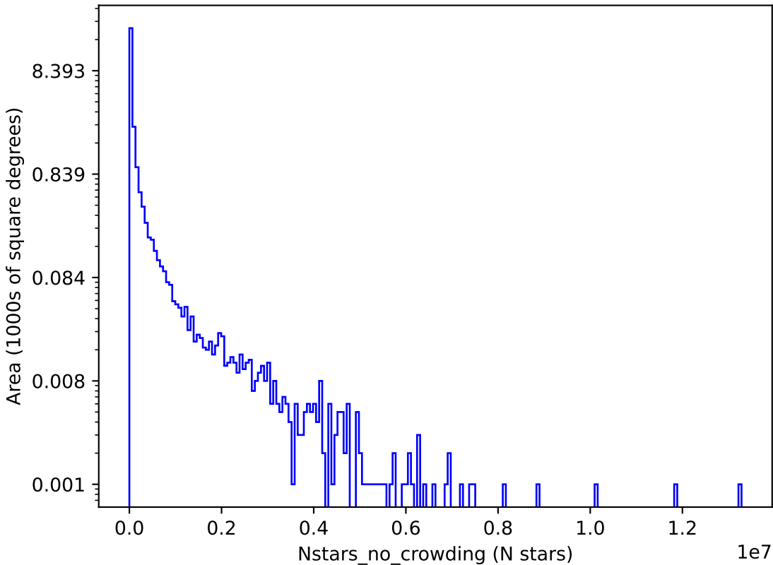
too_10_1v3.4_10yrs g: Nstars_no_crowding
