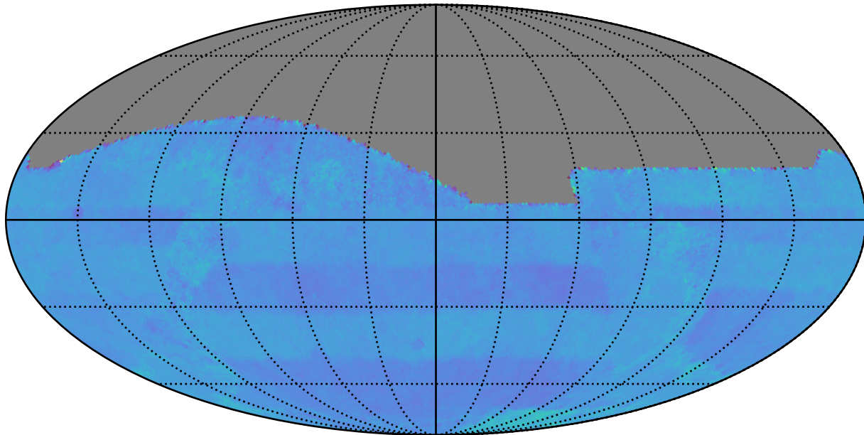
too_10_1v3.4_10yrs : Normalized Proper Motion Uncert @ 24.0
