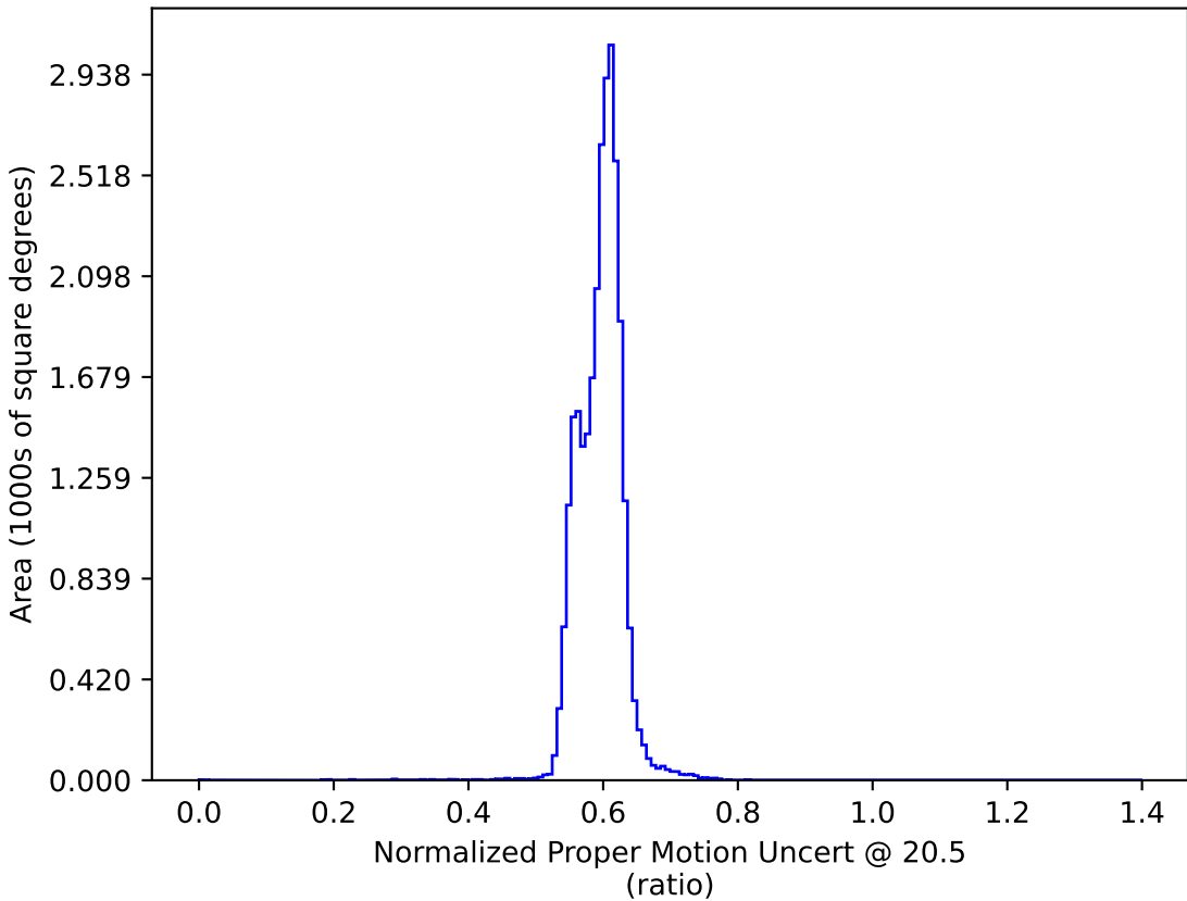
too_10_1v3.4_10yrs : Normalized Proper Motion Uncert @ 20.5
