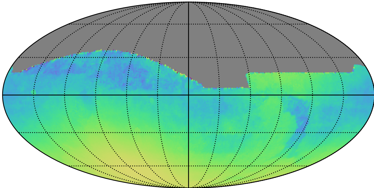
too_10_1v3.4_10yrs : Normalized Parallax Uncert @ 24.0
