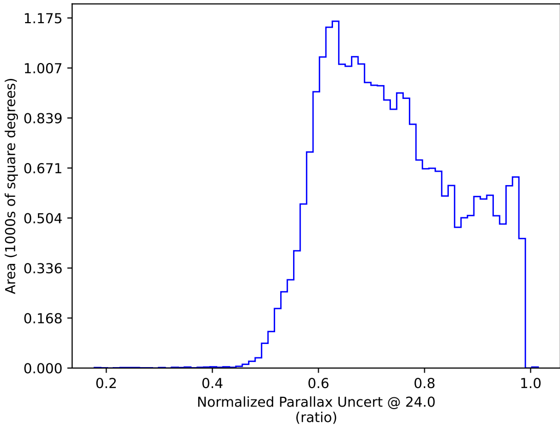
too_10_1v3.4_10yrs : Normalized Parallax Uncert @ 24.0
