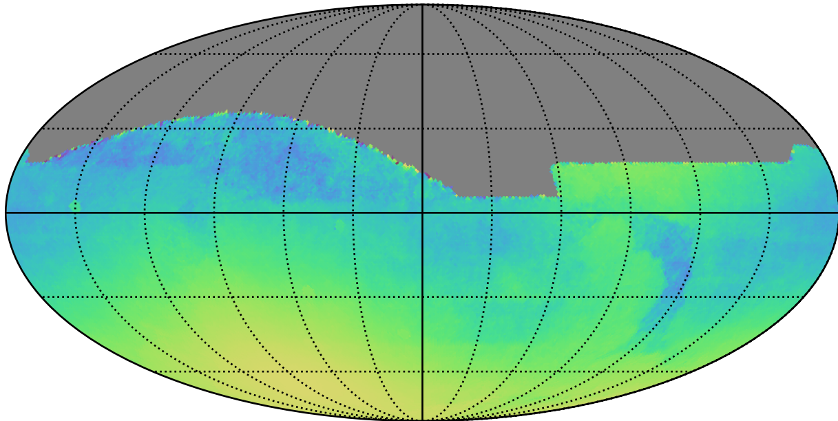
too_10_1v3.4_10yrs : Normalized Parallax Uncert @ 22.4
