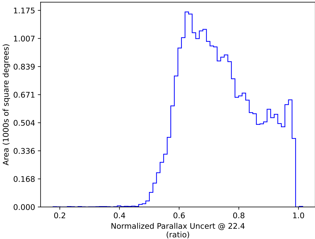
too_10_1v3.4_10yrs : Normalized Parallax Uncert @ 22.4
