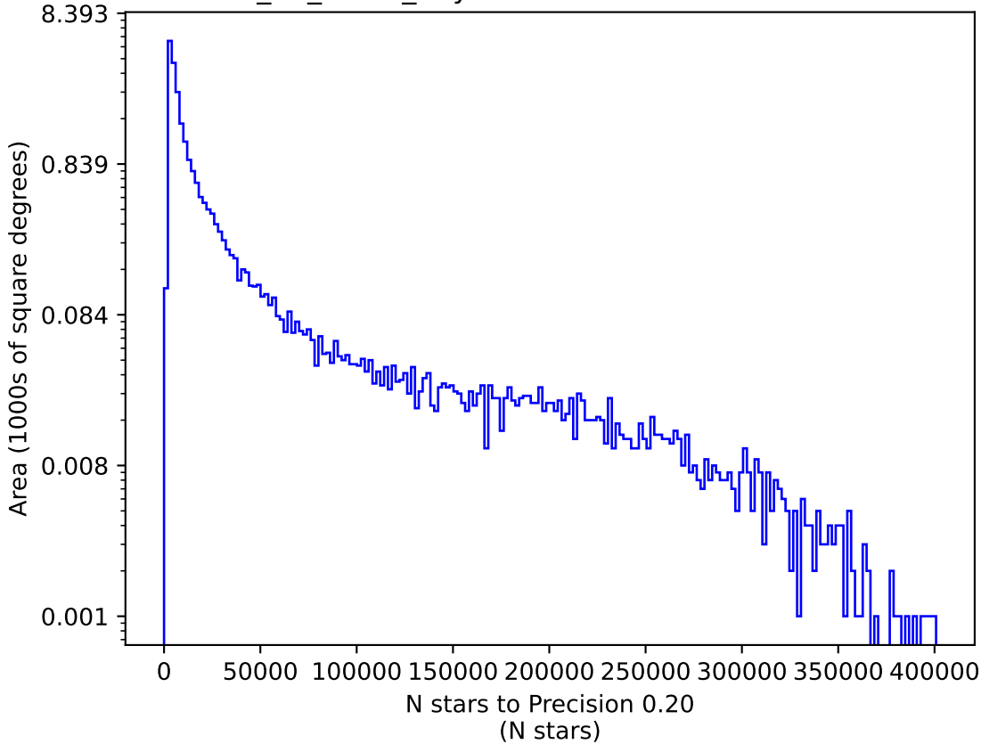
too_10_1v3.4_10yrs u: N stars to Precision 0.20
