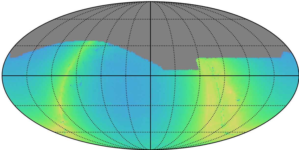
too_10_1v3.4_10yrs r: N stars to Precision 0.20
