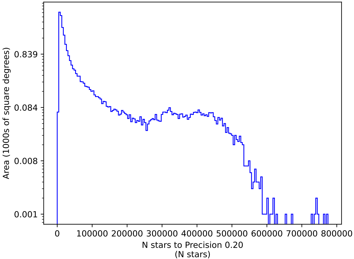
too_10_1v3.4_10yrs r: N stars to Precision 0.20
