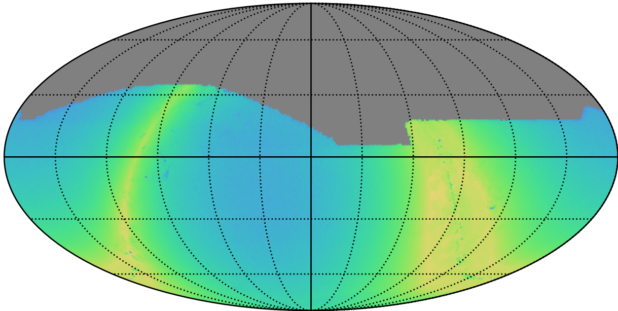
too_10_1v3.4_10yrs i: N stars to Precision 0.20
