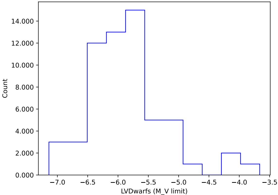
too_10_1v3.4_10yrs gi: LVDwarfs
