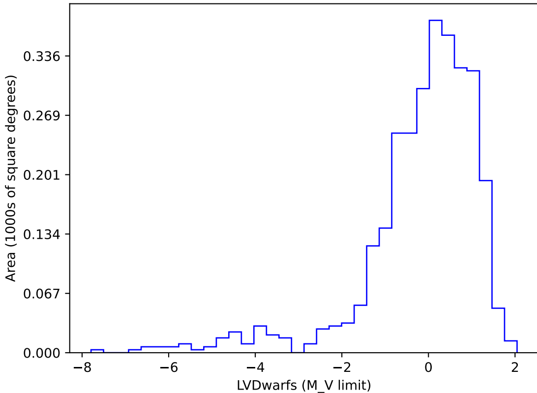
too_10_1v3.4_10yrs gi SCP: LVDwarfs
