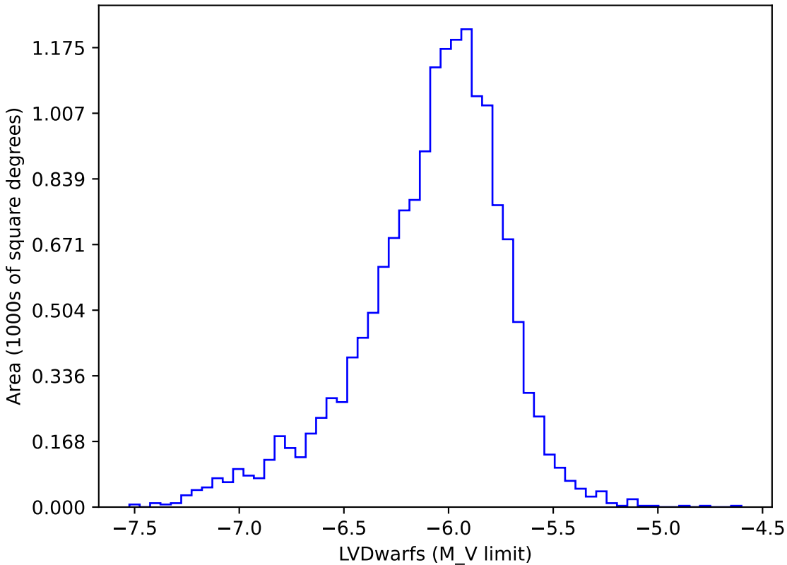
too_10_1v3.4_10yrs gi: LVDwarfs
