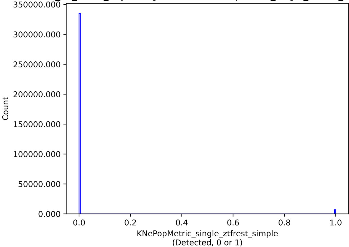
too_10_1v3.4_10yrs single model: KNePopMetric_single_ztfrest_simple
