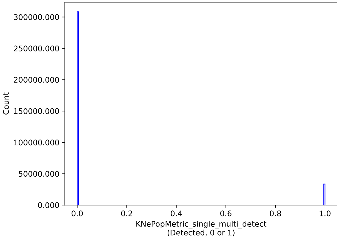
too_10_1v3.4_10yrs single model: KNePopMetric_single_multi_detect
