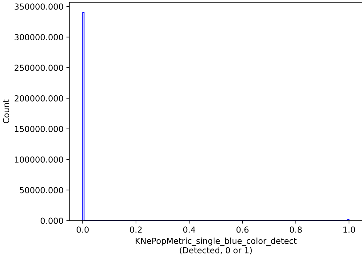
too_10_1v3.4_10yrs single model: KNePopMetric_single_blue_color_detect
