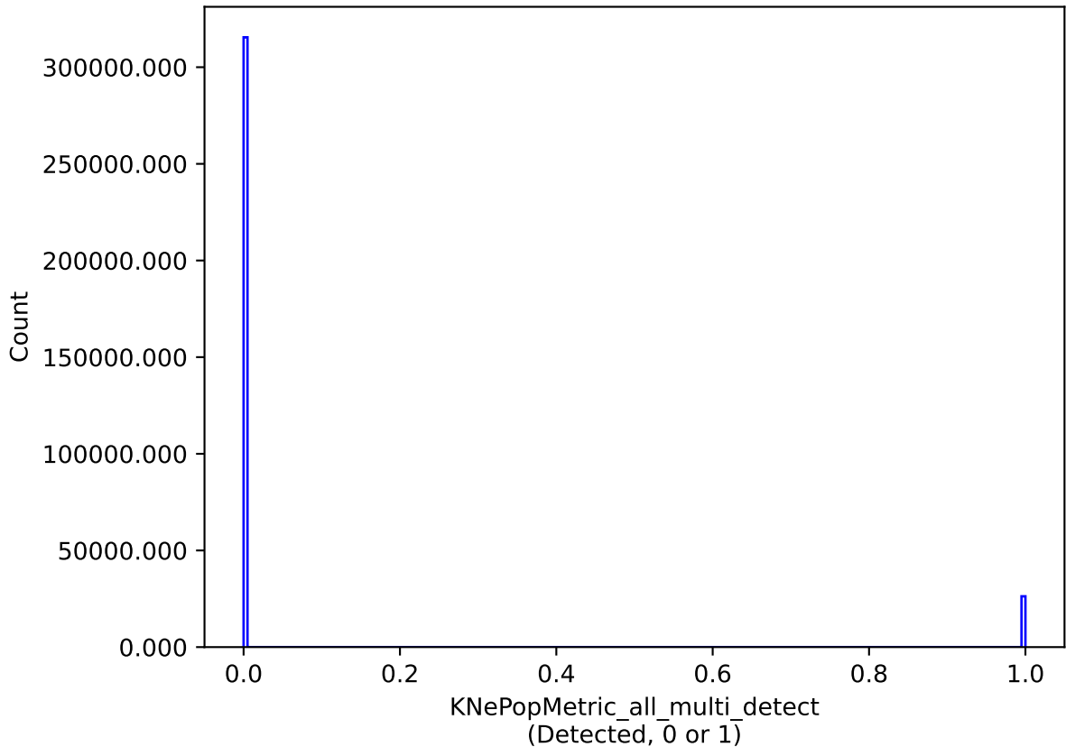
too_10_1v3.4_10yrs all models: KNePopMetric_all_multi_detect
